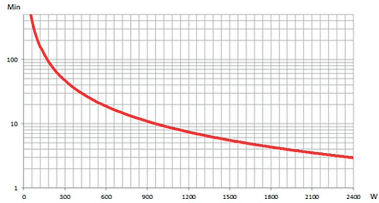
Figure 23. Runtime graph of INFORPRO3000 UPS
