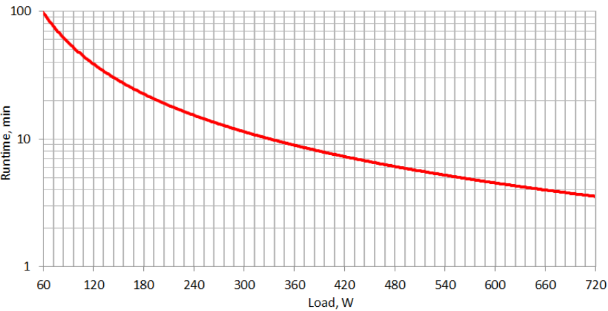
Figure 5. Runtime graph INFO1200 / INFOLCD1200
