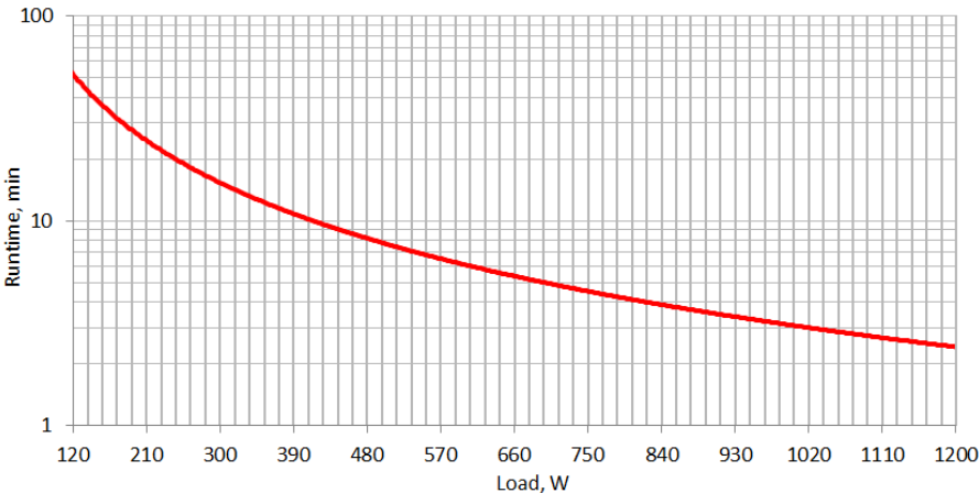
Figure 7. Runtime graph INFO2000 / INFOLCD2000
