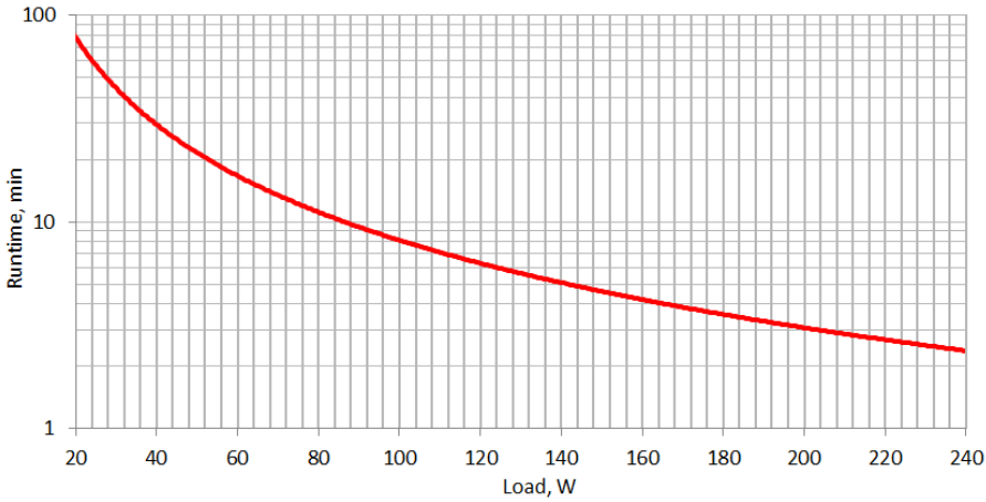
Figure 2. Runtime graph INFO400 / INFOLCD400
