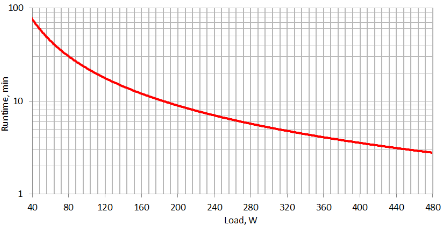
Figure 4. Runtime graph INFO800 / INFOLCD800
