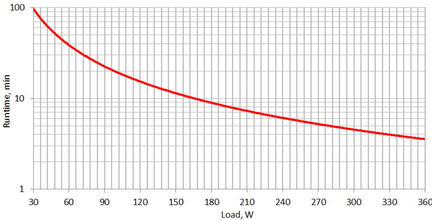
Figure 3. Runtime graph INFO600 / INFOLCD600
