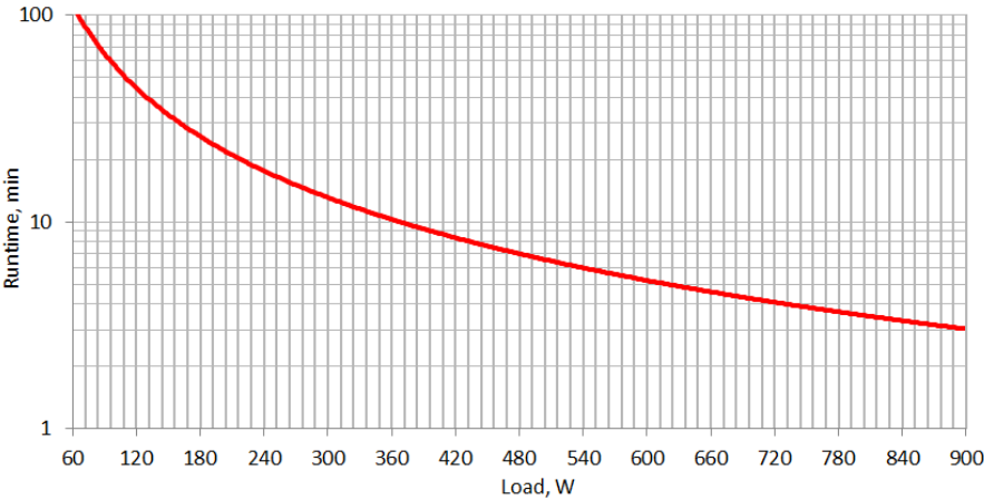
Figure 6. Runtime graph INFO1500 / INFOLCD1500
